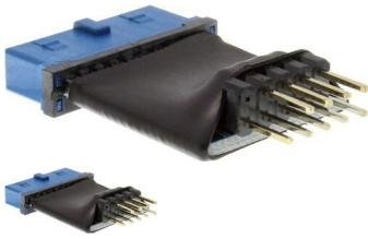
InLine® USB 3.0 zu 2.0 Adapter intern.
